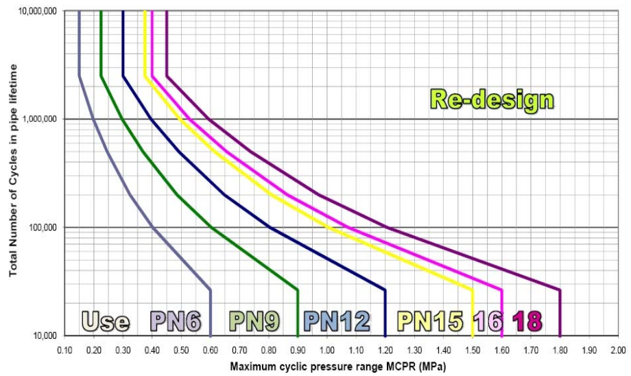
Selection of PVC-M pipe pressure class fatigue applications
