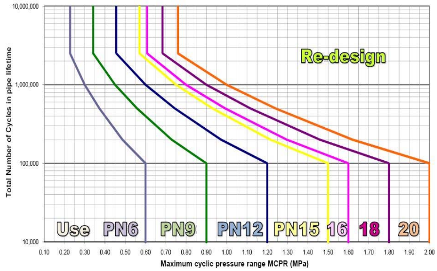
Selection of PVC-U pipe pressure class fatigue applications
