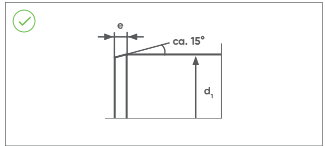
Illustration 7.25 Plug-in joint
