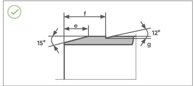
Illustration 7.26 Snap joint
