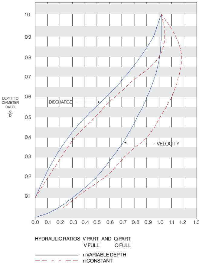
FIGURE C: ADJUSTMENT FACTORS
